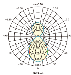
Photometric curves of SPACE 60 P-CL1500U-47W-840-80° ↑ 105° ↓
